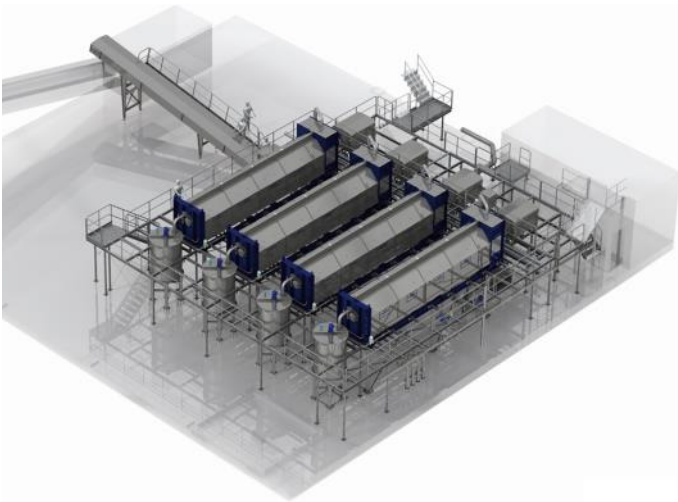
Gryaab, Gothenburg, Sweden - 4 pcs SP-HF13XLE screw press. MF1000 microscreen filtrate filtering and ARU acid rinse equipment. - Largest screw press installation in Europe.
